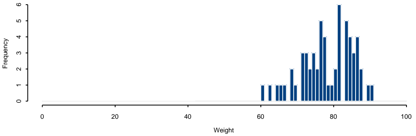
Agreement Weights: False Matched Pairs
