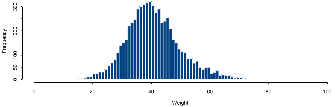
Agreement Weights: False Matched Pairs
